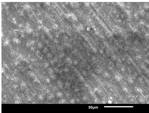
Figure S3. SEM of CNTs from non-treated Al substrate for 10 min growth.
