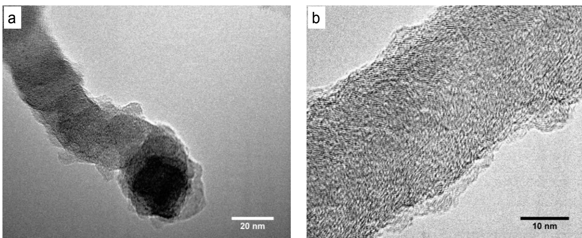
Figure S6. Carbon nanofibers (CNFs) synthesized with surface activation. (a) TEM images of CNFs grown on Al substrates without surface treatment. The average diameter of the CNFs is ca. 26 nm. (b) Zoom-in high resolution TEM images showing the turbostratic nature of the CNFs.
