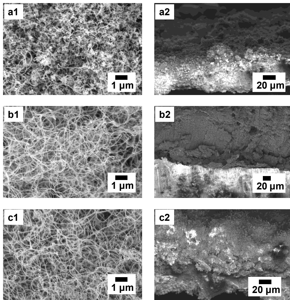
Figure S1. CNT/sa-Al growth results. (a) Top and cross-sectional views of CNTs grown on Al substrate at 400 °C. (b) Top and cross-sectional views of CNTs grown on Al substrate at 500 °C. (c) Top and cross-sectional views of CNTs grown on Al substrate at 600 °C.
