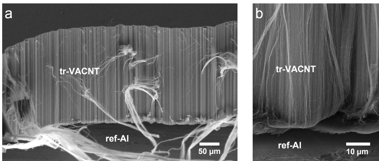
Figure S8. Cross-sectional SEM image of the tr-VACNT/ref-Al sample.
