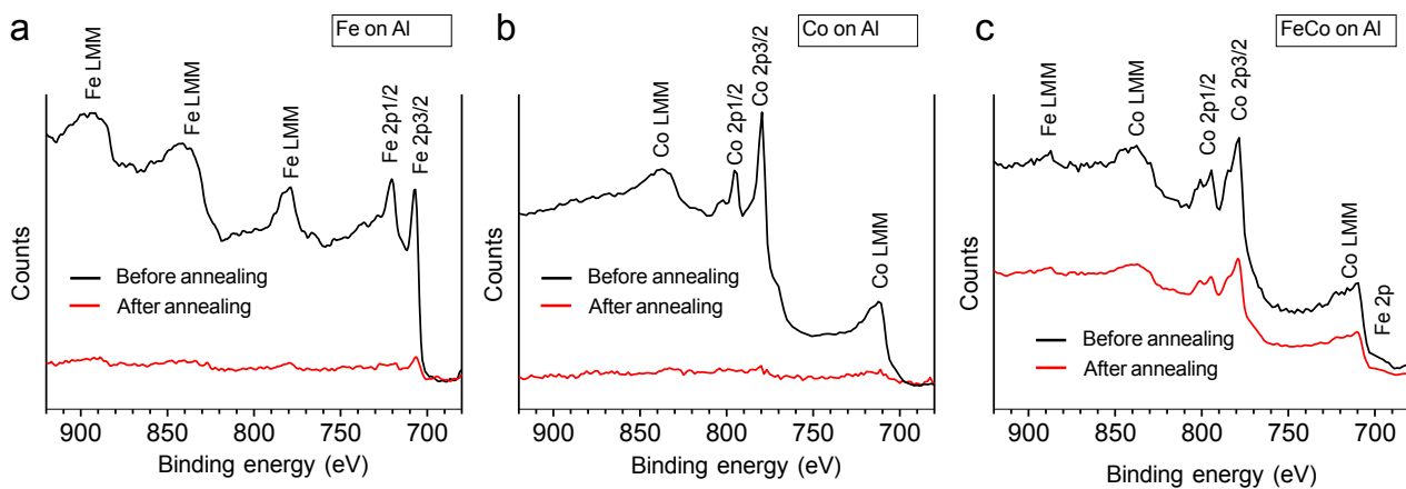
Figure S7. XPS survey spectra of (a) Fe, (b) Co and (c) FeCo catalysts on Al substrate before and after annealing at 500 °C for 30 min.
