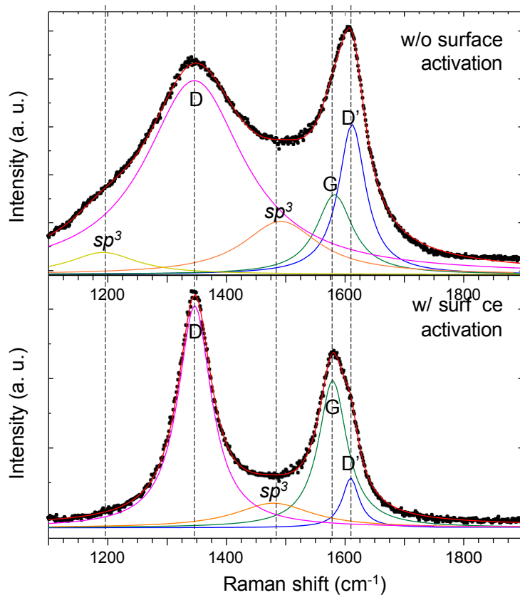
Figure S5. Raman spectra of CNT-Al samples with and without surface activation for the evaluation of I_D/I_G ratio.
