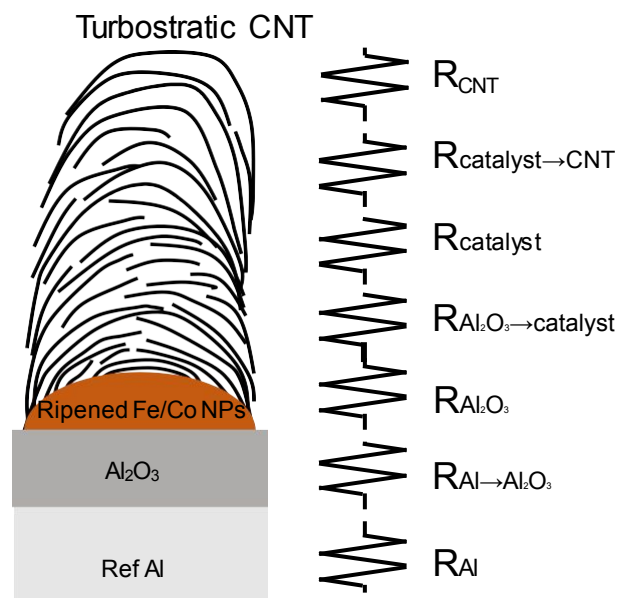
Figure S9. Equivaent circuits for turbostratic CNTs directly grown on ref-Al.
