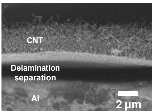
Figure S4. Delamination of CNTs from non-treated Al growth substrate for 2 hours, owing to the large thermal-expansion mismatch between native aluminum oxide and aluminum.
